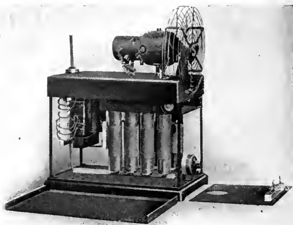
FIG. 15. STANDARD TYPE OF OZONATER (WITH CASING REMOVED) ADAPTED TO LARGE OFFICES, COLD STORAGE ROOMS, FACTORIES, AUDITORIUMS, HOSPITALS, ETC.
